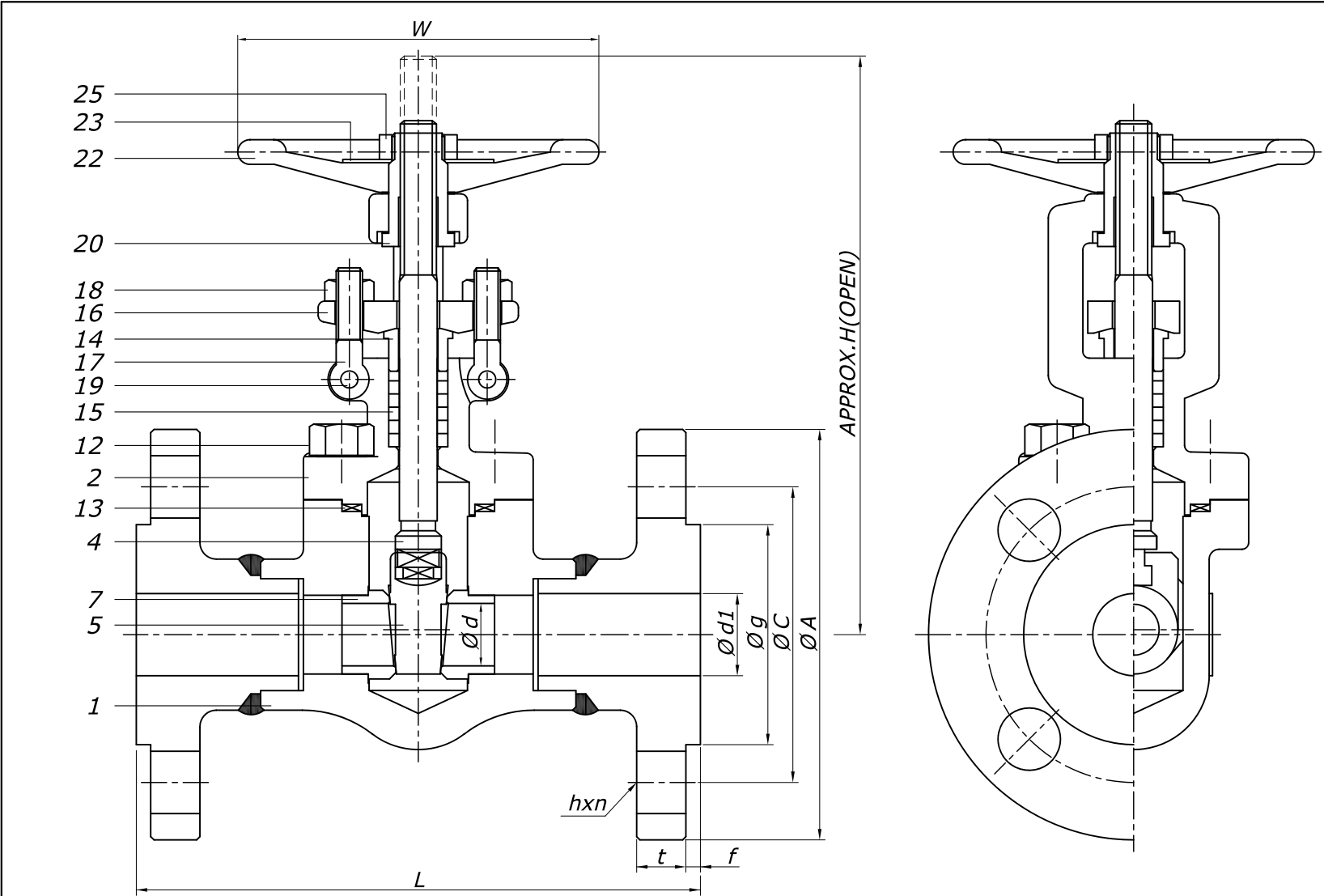
DIMENSIONS (UNIT: mm)
