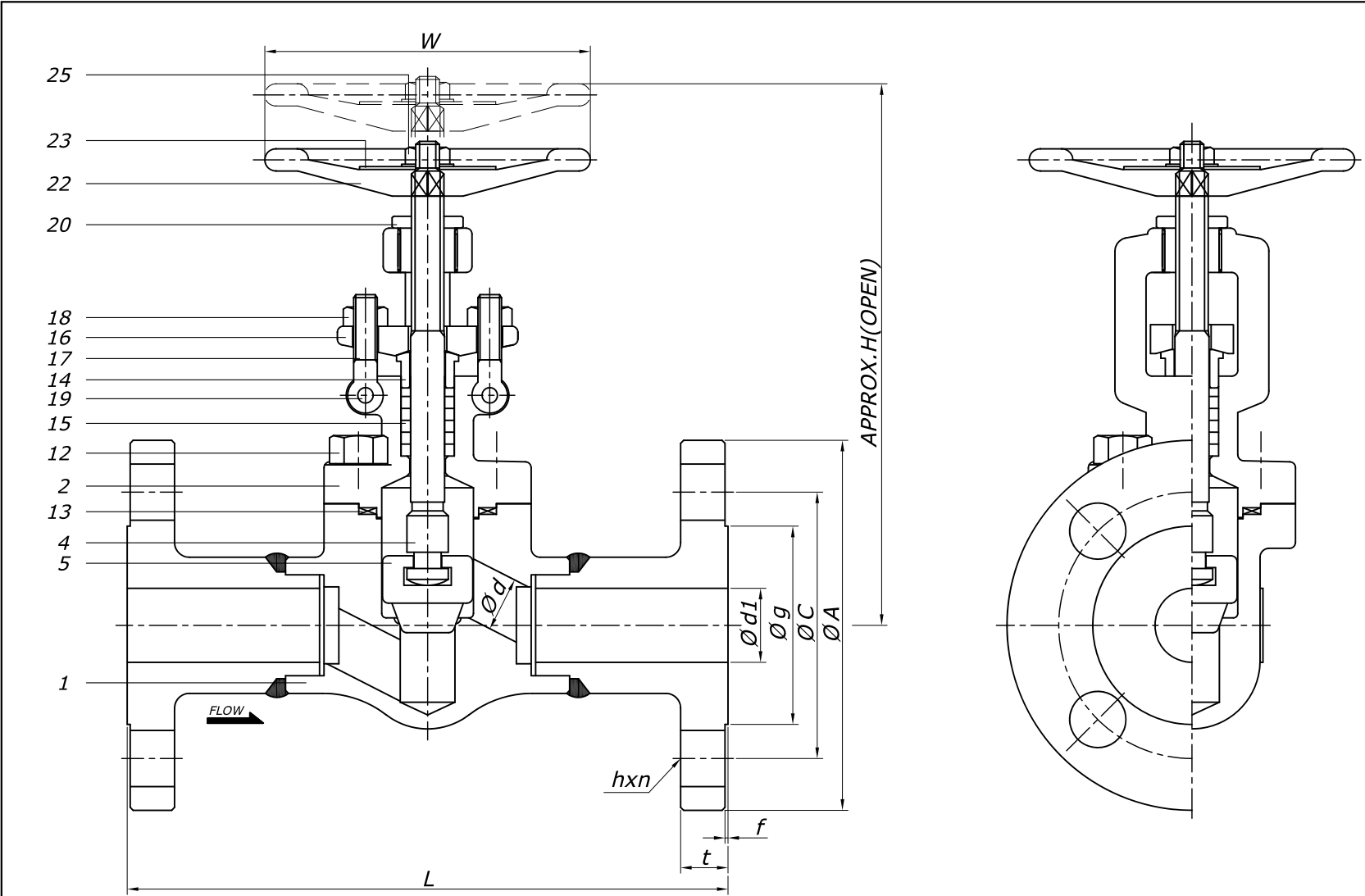
DIMENSIONS (UNIT: mm)
